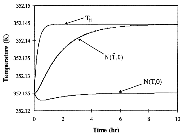
Figure 4. Response of one-degree-of-freedom nonlinear PID controller showing tracking of model error between approximate and true process.
