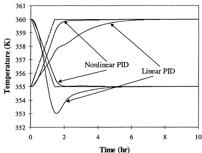
Figure 3. Response to step changes, both increase and decrease, for two-degree-of-freedom linear and nonlinear PID controllers.
