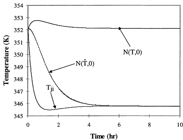
Figure 5. Response of one-degree-of-freedom nonlinear PID controller to unmeasured 20% drop in F , demonstrating process monitoring and quantification of model error.
